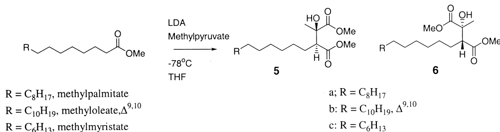
Scheme 1. Aldol condensation of fatty acid esters with methyl pyruvate.
