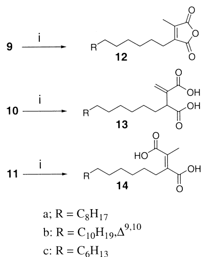
Scheme 3. Hydrolysis of esters. Reagents: (i) a. 1 N NaOH, CH 3 OH–THF–H 2 O, 80 °C; b. 4 N HCl.
