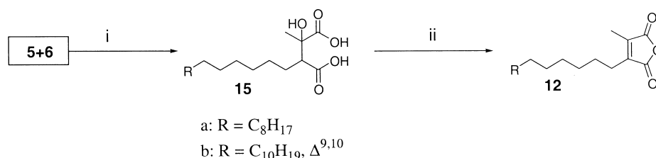
Scheme 4. Modified synthesis of chaetomelic acids A and B. Reagents: (i) LiOH, THF–H 2 O; (ii) Ac 2 O, reflux.
