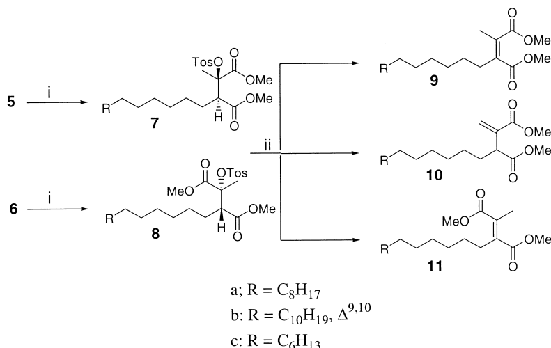
Scheme 2. β-Elimination reactions of tosylated aldol products. Reagents: (i) p -toluenesulfonic anhydride, CH 2 Cl 2 , C 5 H 5 N, 2,6-di- tert -butyl-4-methylpyridine, 40 °C; (ii) toluene, DBU, reflux.
