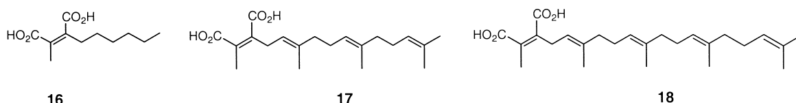
Figure 2. Structures of synthetic and natural chaetomelic acid analogues (diacid form).
